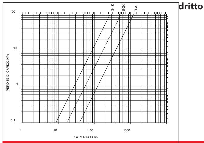
dritto 3/8" - 1/2" QmN 175
