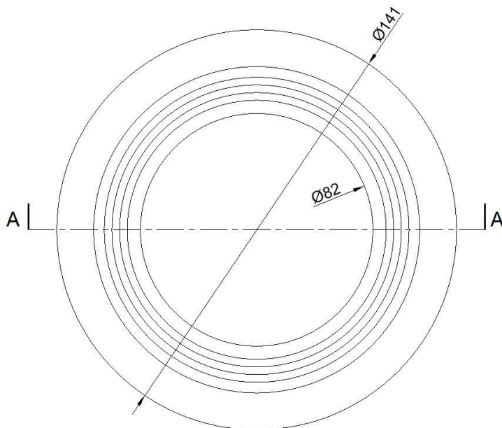
VISTA ZENITALE ZENITHAL VIEW
